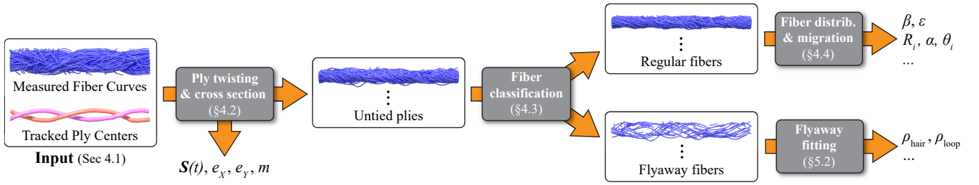
Figure 4: Our parameter fitting pipeline. This pipeline is approximately in the opposite order of the procedural yarn generation algorithm (Algorithm 1) since it is fitting parameters.
